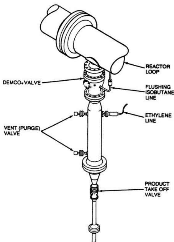
Figure 5: Typical Settling Leg Assembly for Phillips Polyethylene Reactor
